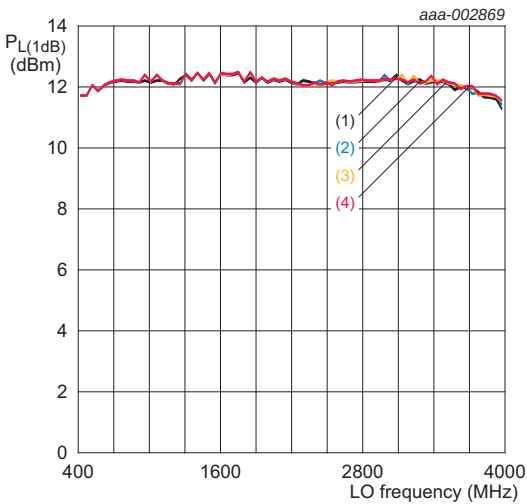
Fig 13. P_L(1dB) versus f_{lo} and V_{CC}
