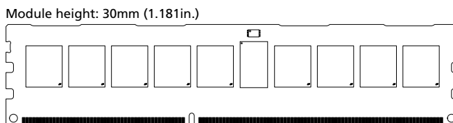
Figure 1: 240-Pin RDIMM (MO-269 R/C B1)
