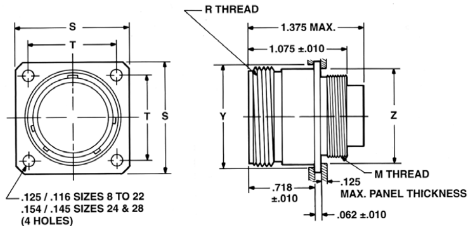
THREADED COUPLING Class K Stainless Steel Pyle FPK-17XX* Series MS27613KXXTXX* Military Class K
