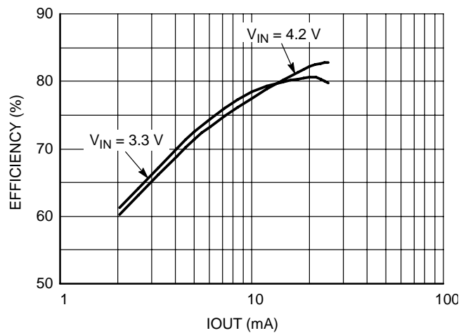
Figure 15. Efficiency vs. I_{OUT} V_{OUT} = 18\text{ V} , L = 22\text{ }\mu\text{H} , VLF 4012-220
