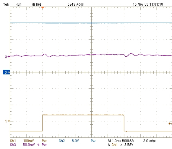
Figure 18. Line Transient Rejection, 1 V_{IN} 3.5 to 3.7 V, 2 V_{OUT} , 5V/div DC, 3 I_{OUT} , 50mA/div AC, T = 1 ms/div
