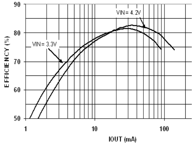
Figure 11. Efficiency vs. I_{OUT} V_{OUT} = 6.0\text{ V} , L = 22\text{ }\mu\text{H} , VLF 4012-220
