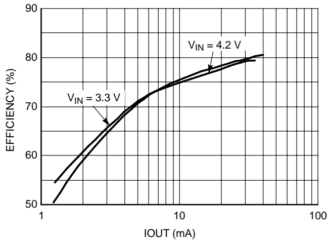
Figure 12. Efficiency vs. I_{OUT} V_{OUT} = 12\text{ V} , L = 10\text{ }\mu\text{H} , VLF 4012-100
