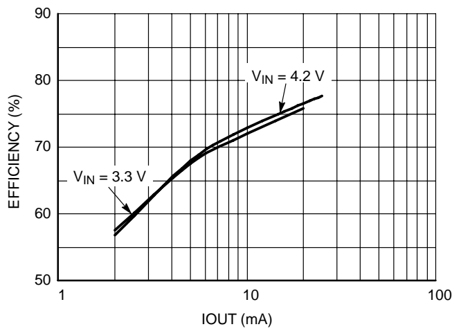
Figure 14. Efficiency vs. I_{OUT} V_{OUT} = 18\text{ V} , L = 10\text{ }\mu\text{H} , VLF 4012-100
