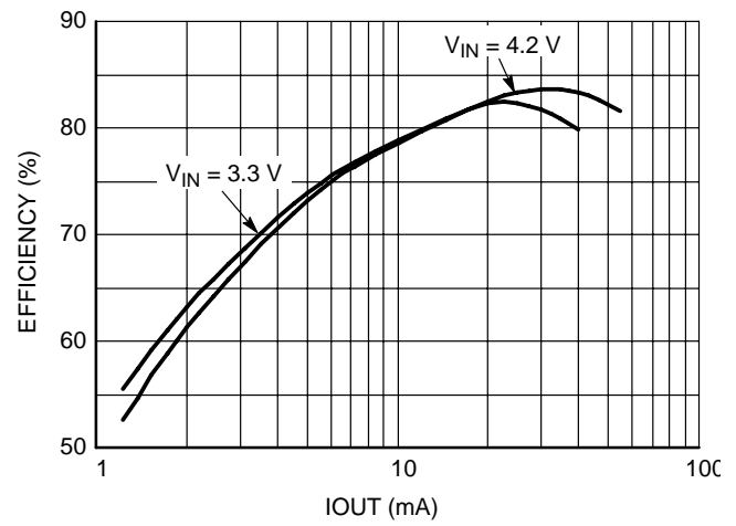
Figure 13. Efficiency vs. I_{OUT} V_{OUT} = 12\text{ V} , L = 22\text{ }\mu\text{H} , VLF 4012-220
