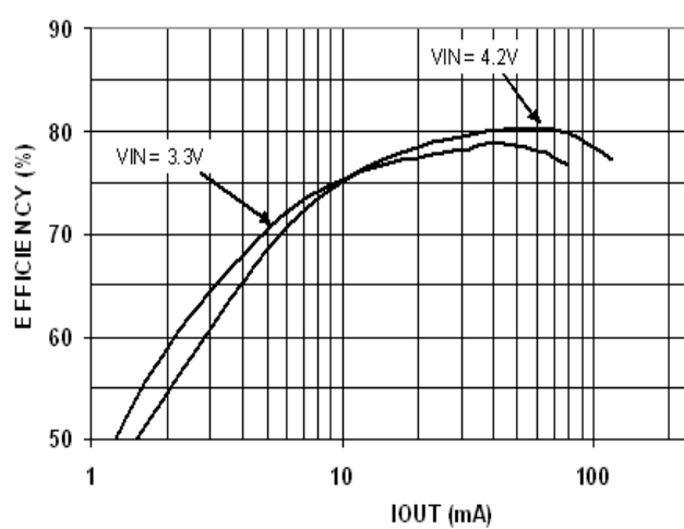
Figure 10. Efficiency vs. I_{OUT} V_{OUT} = 6.0\text{ V} , L = 10\text{ }\mu\text{H} , VLF 4012-100
