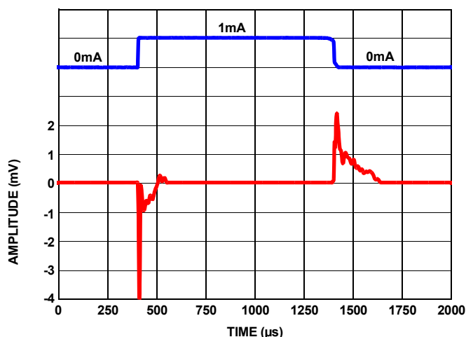
FIGURE 11. LOAD TRANSIENT RESPONSE AT 1mA LOAD AT 1\mu F
