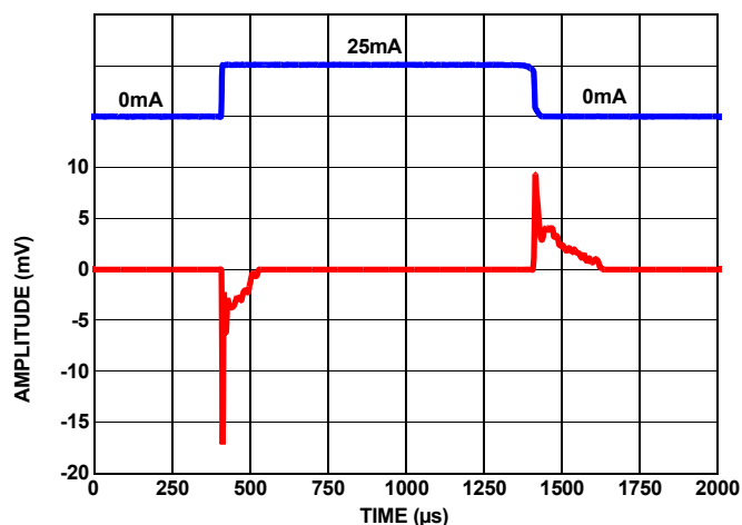
FIGURE 10. LOAD TRANSIENT RESPONSE AT 25mA LOAD AT 1\mu F
