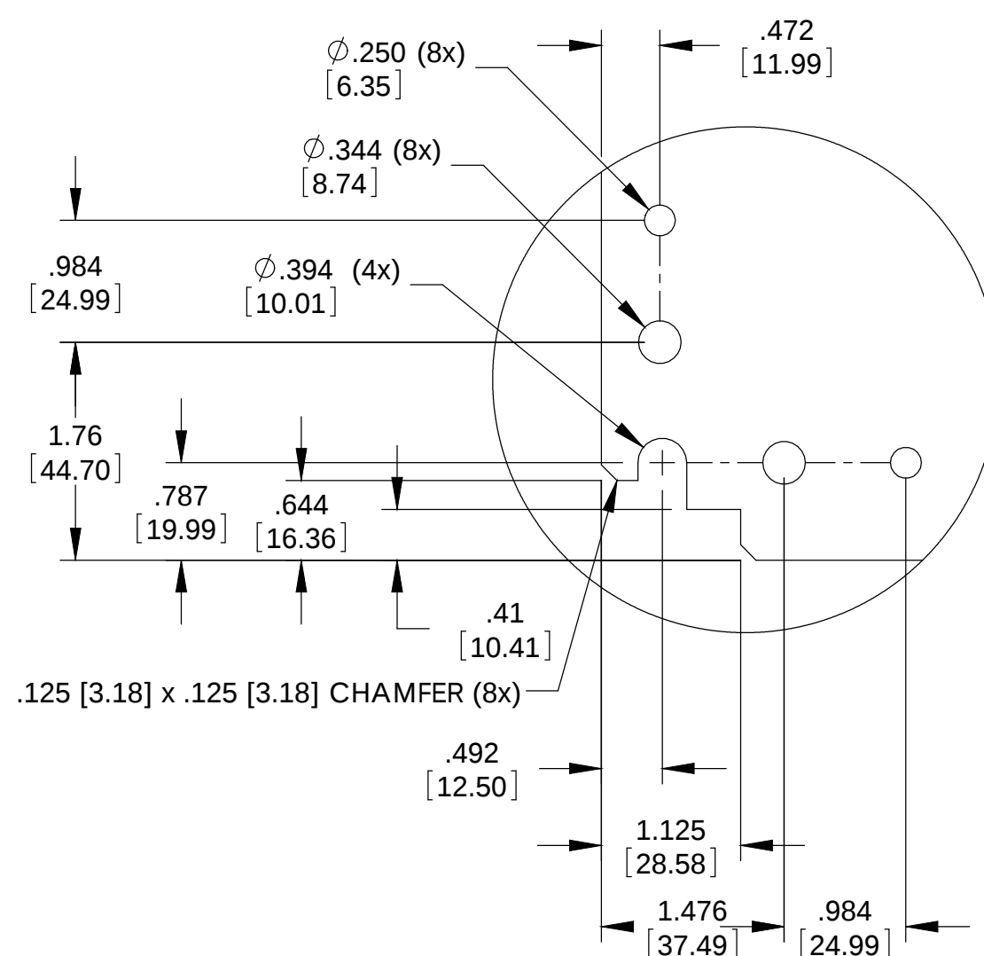
DETAIL A SCALE 2 : 2.75
