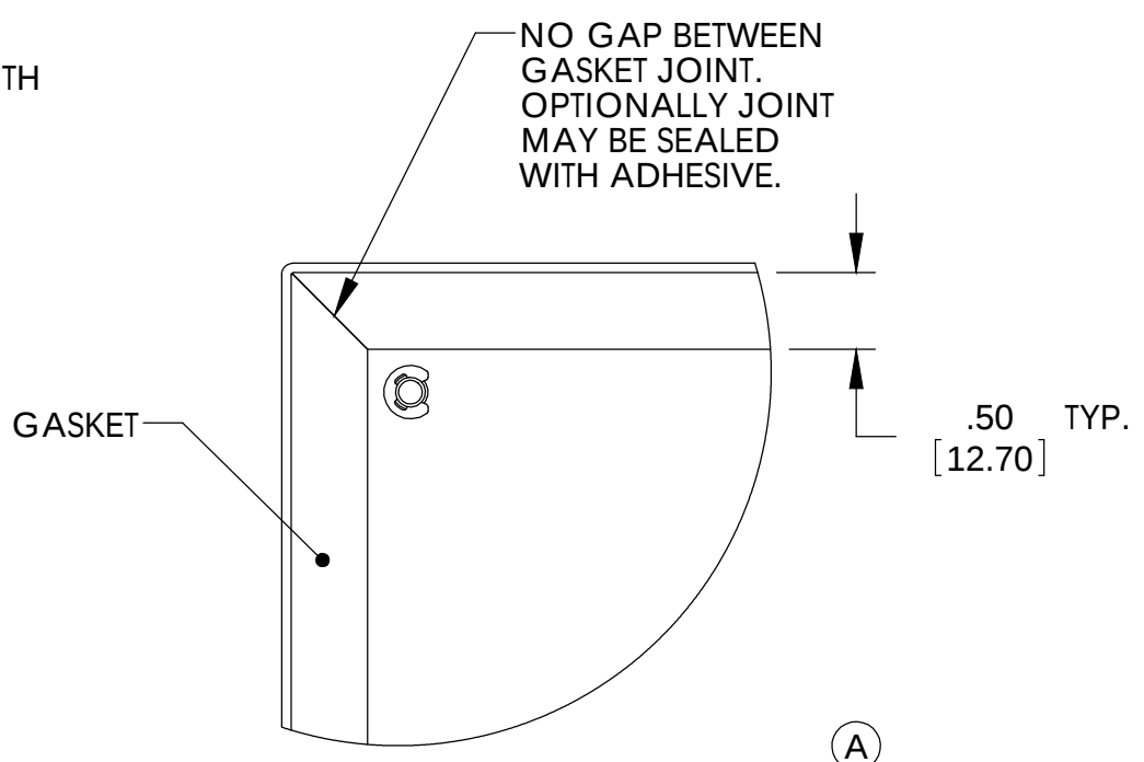
DETAIL D SCALE 2 : 2.75
