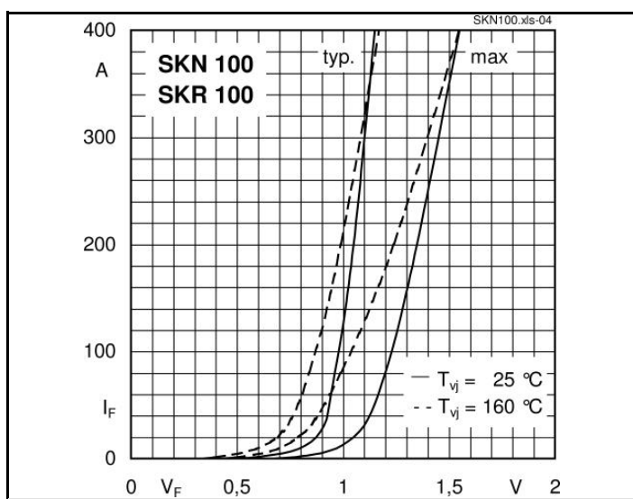
Fig. 5 Forward characteristics
