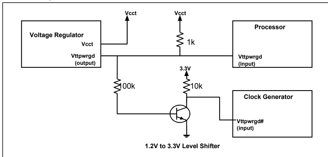
Figure 3. VTPWRGD System-Level Connections
