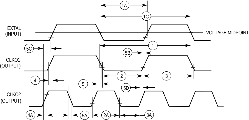
Figure 10-2. Clock Timing
