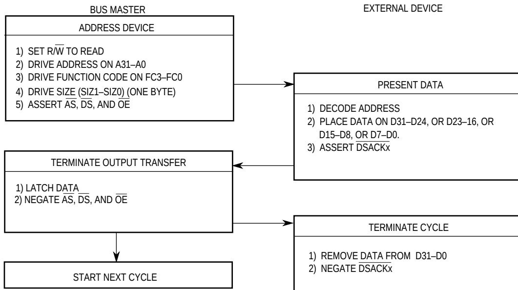
Figure 4-16. Byte Read Cycle Flowchart
