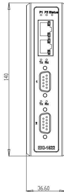
Figure 2.7 Front View of EKI-1521/1522
