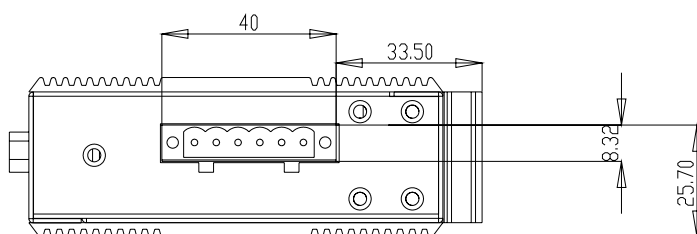
Figure 2.10 Top View of EKI-1521/1522
