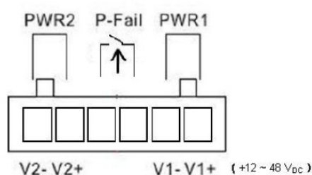
Figure 2.18 Power Connector
