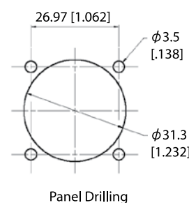
Panel Drilling
