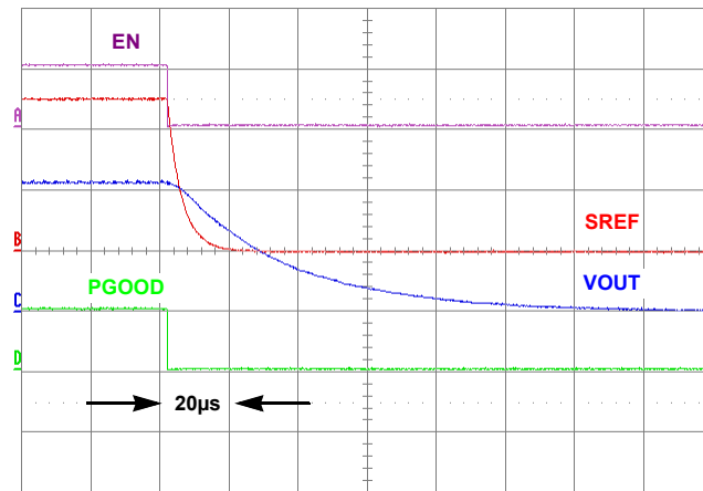
FIGURE 18. SHUT-DOWN, V_{IN} = 12.6V , V_{OUT} = 1.05V , I_{LOAD} = 50mA
