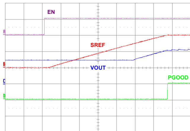
FIGURE 17. START-UP INTO 750mV PRE-BIASED OUTPUT, V_{IN} = 12.6V , V_{OUT} = 1.05V , I_{LOAD} = 10A
