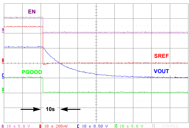
FIGURE 19. SHUT-DOWN, V_{IN} = 12.6V , V_{OUT} = 1.05V , I_{LOAD} = OPEN-CIRCUIT
