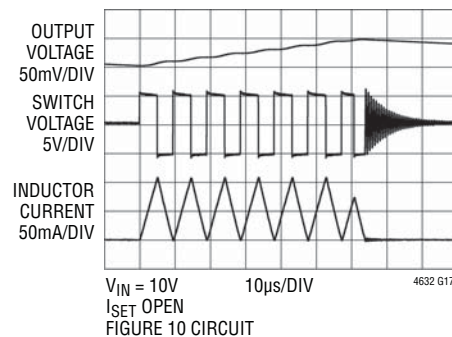
Operating Waveforms
