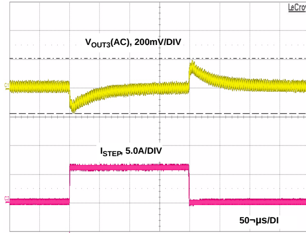
FIGURE 12. PWM3 LOAD TRANSIENT RESPONSE (LOAD STEP FROM 3A TO 9A)
