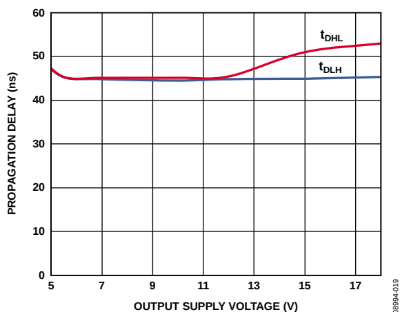
Figure 13. Typical Propagation Delay vs. Output Supply Voltage, V_{DD1} = 5 V
