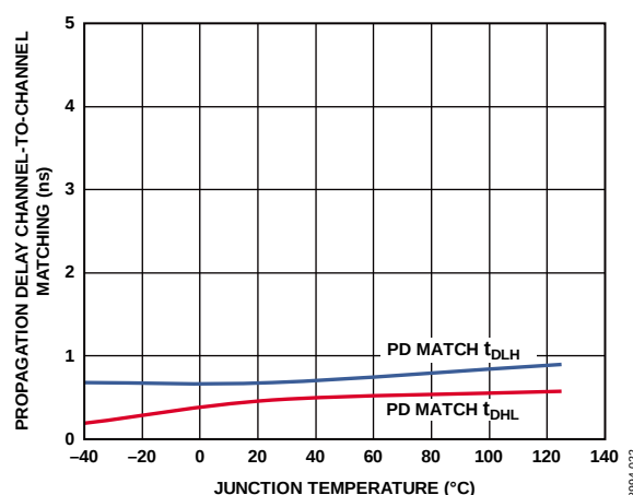
Figure 16. Typical Propagation Delay Channel-to-Channel Matching vs. Temperature, V_{DD2} = 10 V
