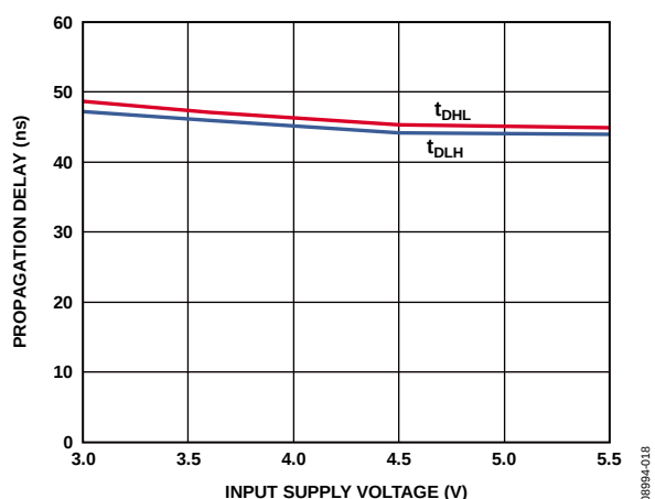
Figure 12. Typical Propagation Delay vs. Input Supply Voltage, V_{DD2} = 10 V
