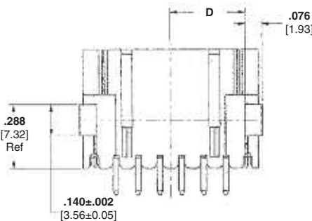
Section K-K
