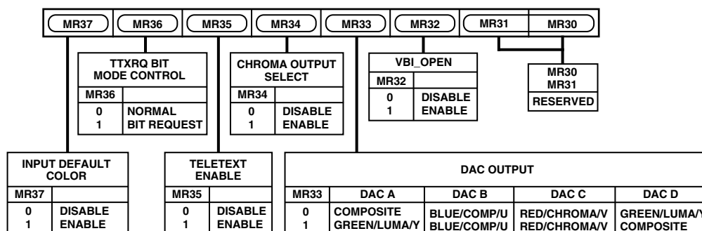
Figure 41. Mode Register 3
