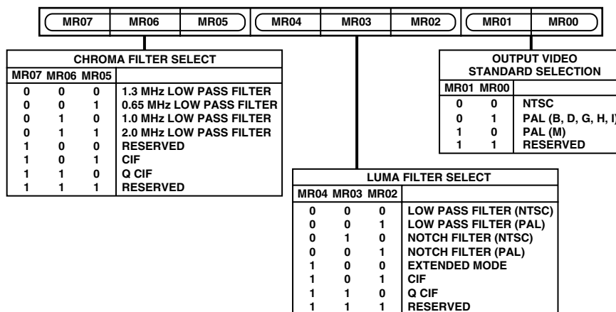
Figure 38. Mode Register 0
