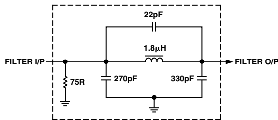
Figure 79. Output Filter
