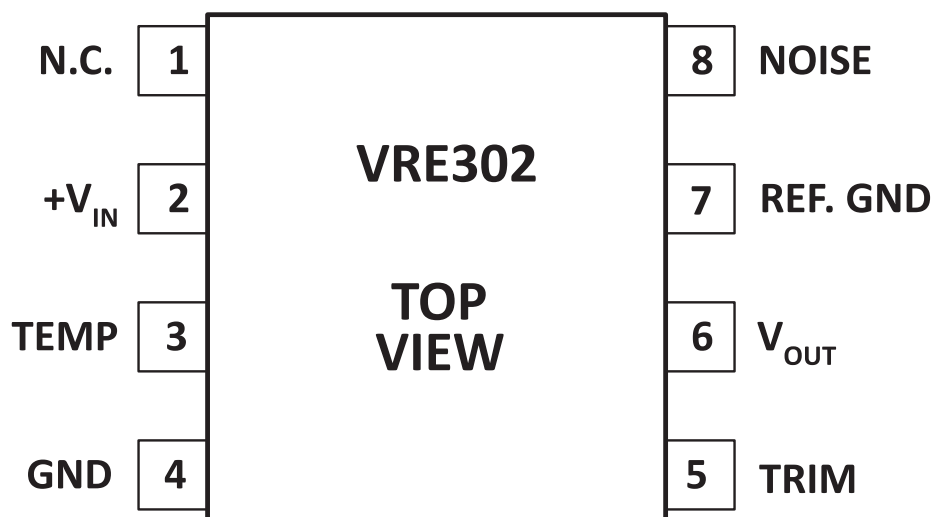
Figure 8: Pin Configuration
