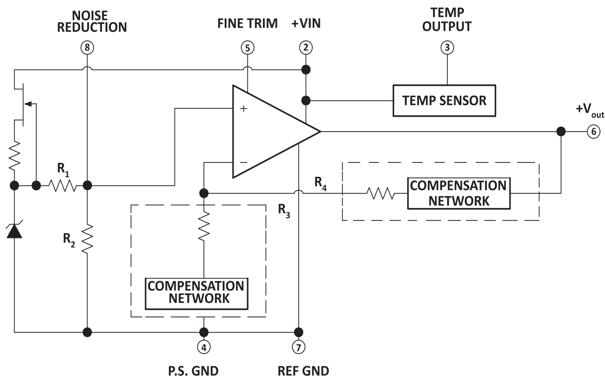
Figure 7: Block Diagram
