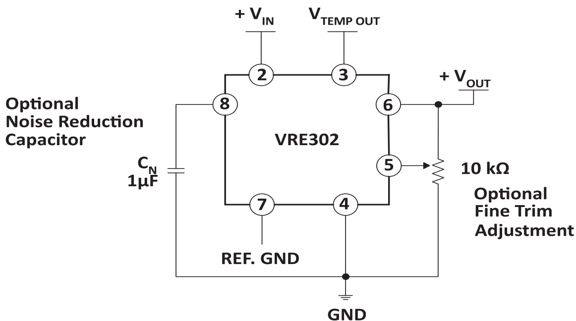
Figure 1: Typical Connection
