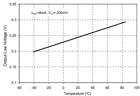
Receiver Output Low Voltage vs Temperature
