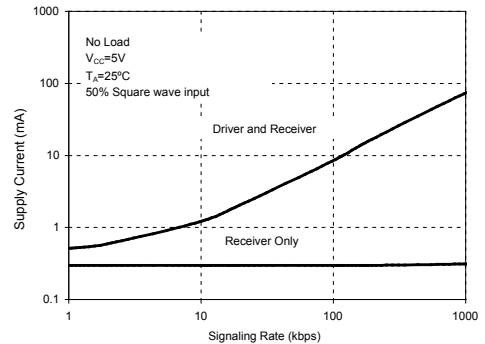
Supply Current vs Signaling Rate (SP3083-SP3085)
