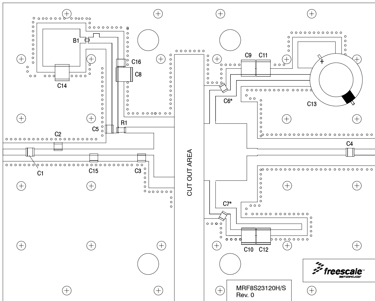
Figure 1. MRF8S23120HR3(HSR3) Test Circuit Component Layout
