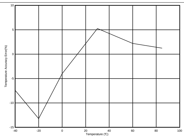
Figure 3. Temperature Accuracy
