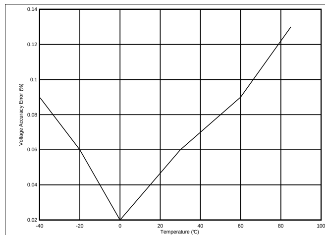
Figure 2. Voltage Accuracy
