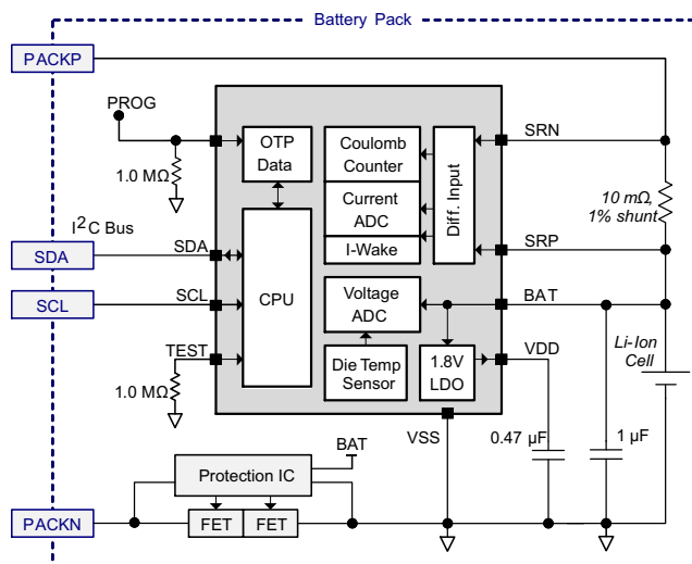
Simplified Schematic
