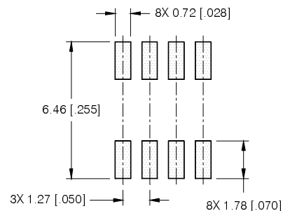
FOOTPRINT
