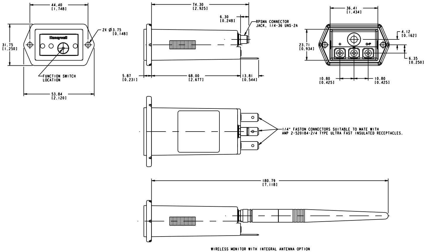
Figure 1. WPMM Dimensions
