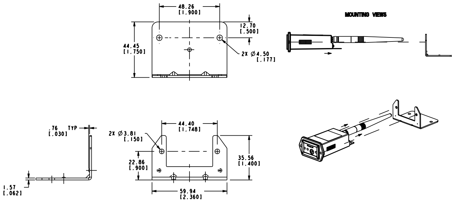
Figure 4. WPR1 Retainer Dimensions
