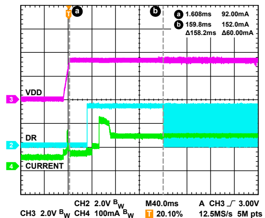
Figure 44. Transient Current Demand, Startup
