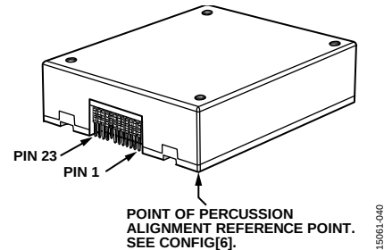
Figure 40. Point of Percussion Reference Point
