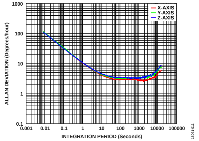
Figure 11. Gyroscope Allan Deviation, ADIS16497-3
