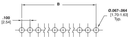
Recommended PC Board Hole Layout
