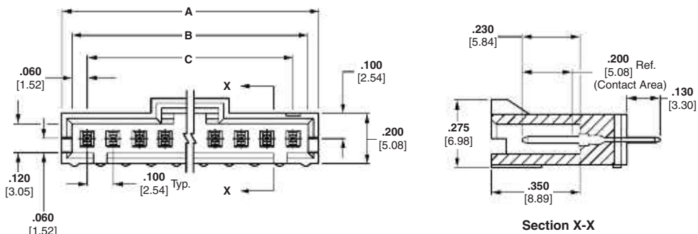
Section X-X
