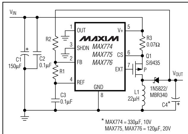
Figure 4. Nonbootstrapped Operation ( V_{IN} > 4.5V )
