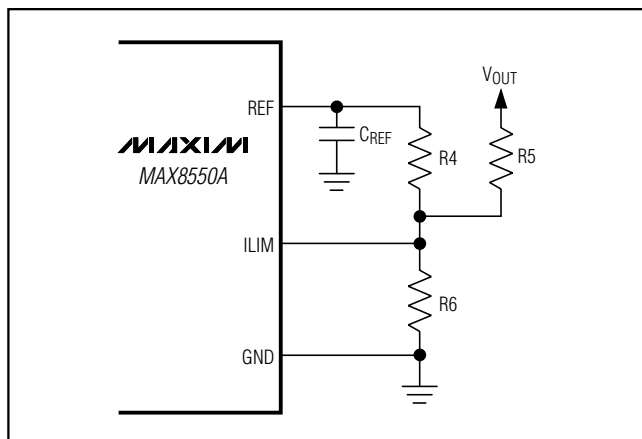
Figure 7. Foldback Current Limit
