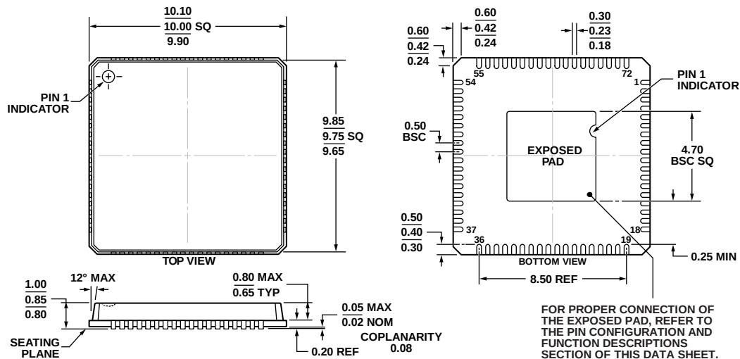
Figure 44. 72-Lead Lead Frame Chip Scale Package [LFCSP_VQ] 10 mm × 10 mm, Very Thin Quad (CP-72-1) Dimensions shown in millimeters
