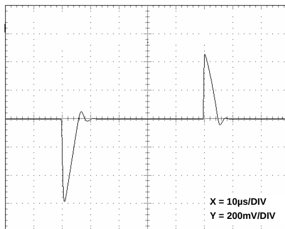
FIGURE 37. LINE TRANSIENT RESPONSE, NO CAPACITIVE LOAD
