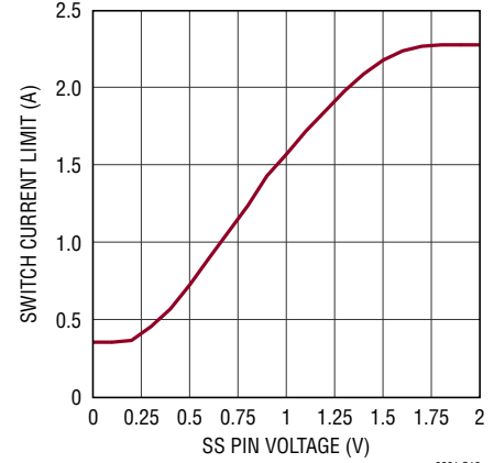
Soft-Start
