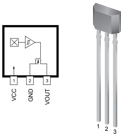
Package UA, 3-pin SIP
