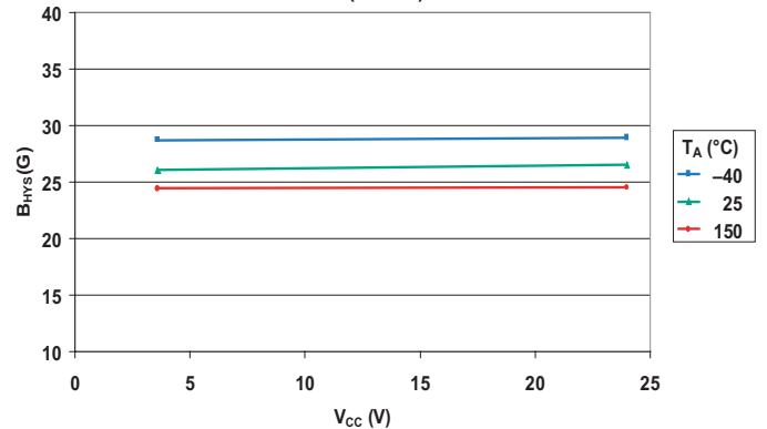
Hysteresis versus Supply Voltage (A3242)
