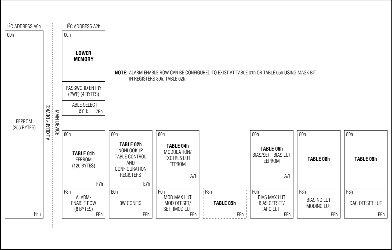
Figure 21. Memory Organization
