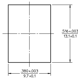
RECOMMENDED MOUNTING CUTOUT FOR .063" THICK PANEL
