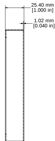
SECTION MM-MM
