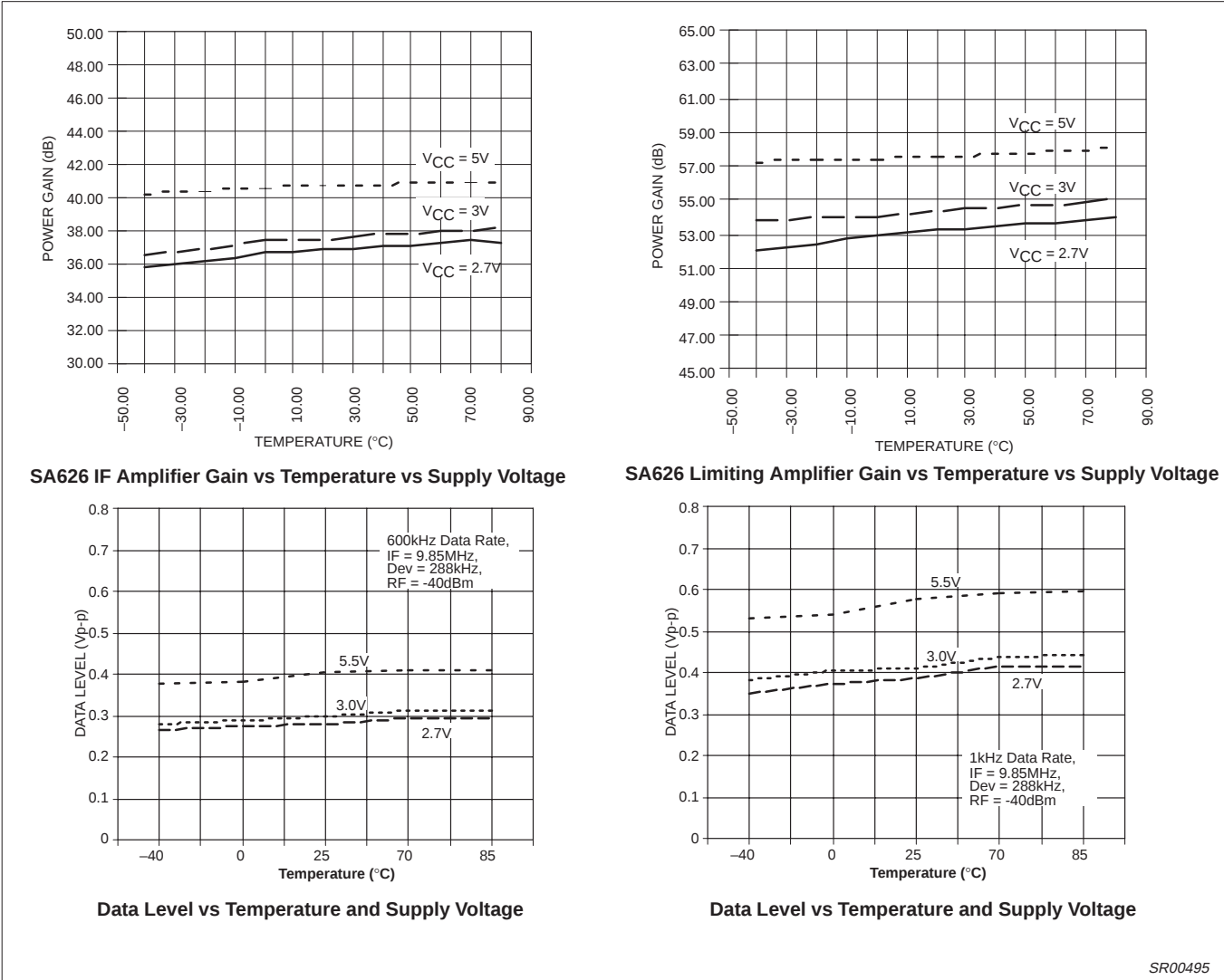
Figure 5. Performance Characteristics
