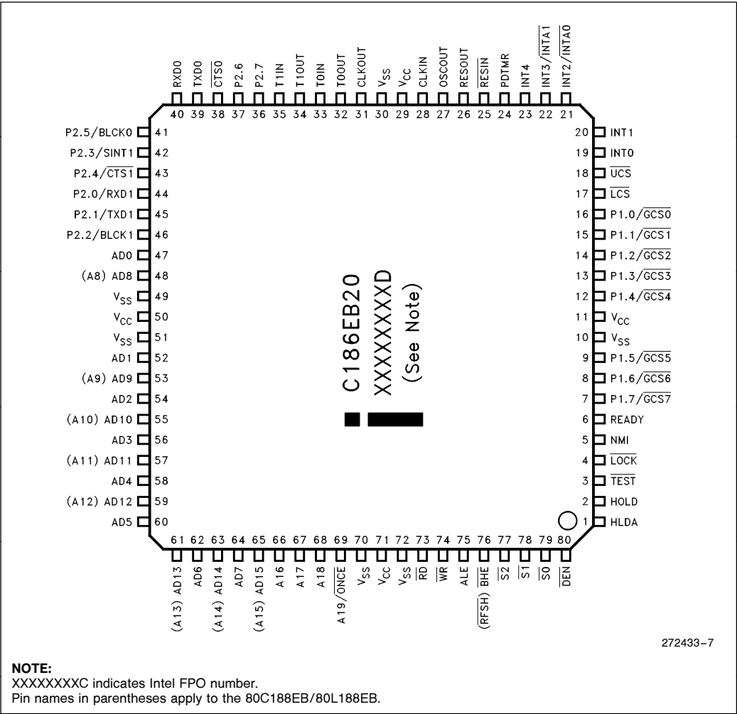
Figure 6. SQFP Package
