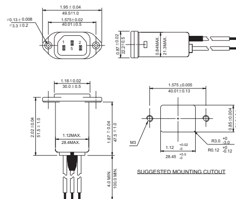
SUGGESTED MOUNTING CUTOUT
