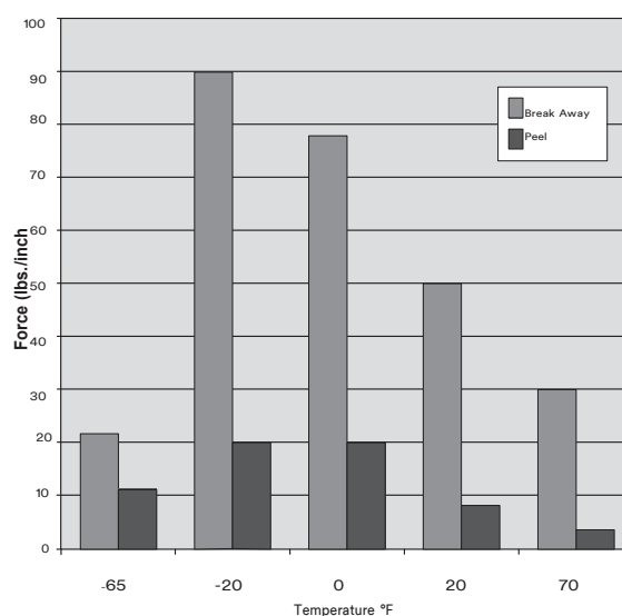
Figure 1. T-Peel Performance vs. Temperature (3M™ VHB™ Adhesive Transfer Tape F9473PC on Aluminum)
