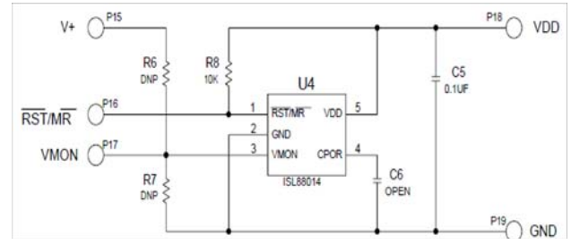
FIGURE 20. ISL88014EVAL1Z
