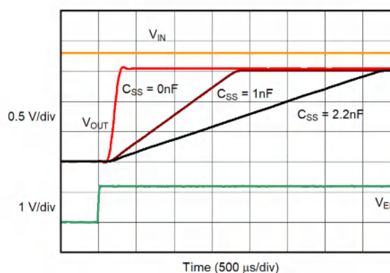
Figure 6-44. Turn-On Response
