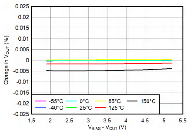
Figure 6-23. V_{BIAS} Line Regulation
