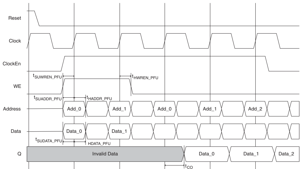
Figure 11-41. PFU Based Distributed Single Port RAM Timing Waveform – with Output Registers
