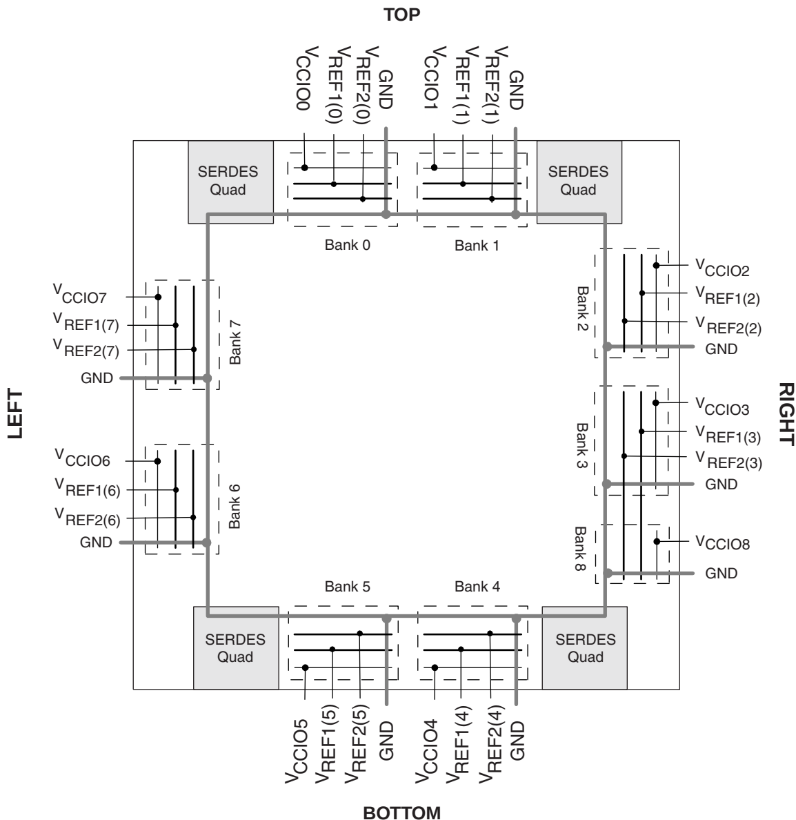
Figure 2-38. LatticeECP2M Banks
