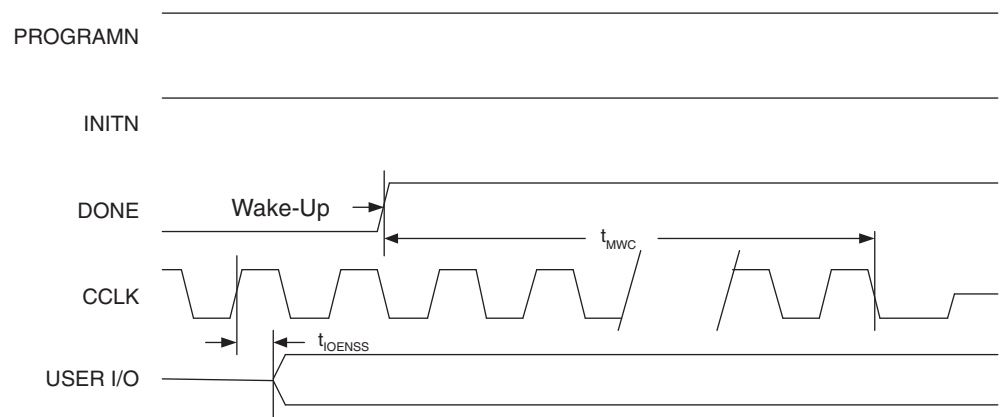
Figure 3-19. Wake-Up Timing
