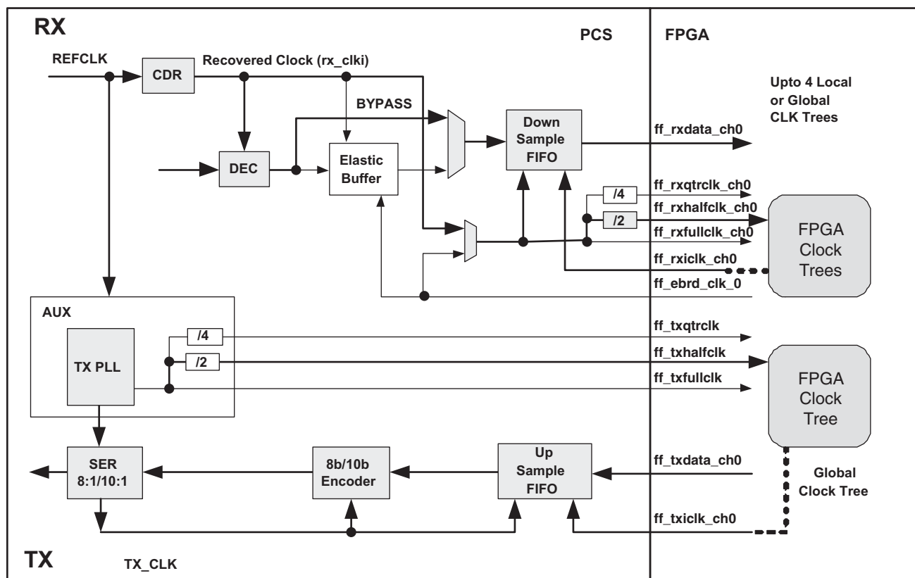
Figure 8-36. 16/20 Bit, DS FIFO NOT Bypassed
