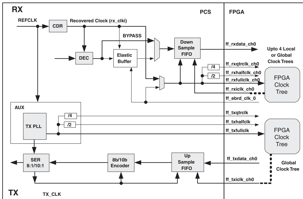
Figure 8-34. 8b10b, EB FIFO Bypassed
