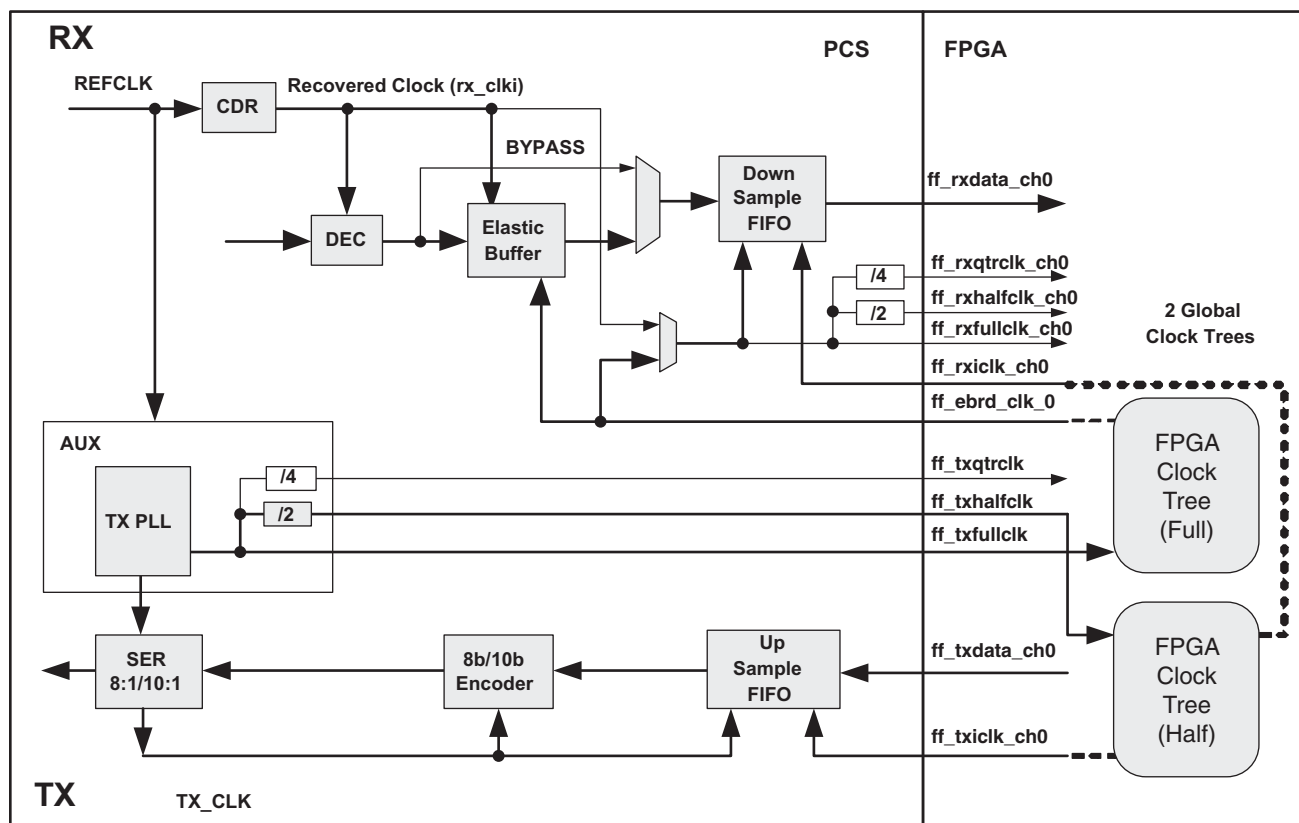
Figure 8-35. 16/20bit, EB and DS FIFOs NOT Bypassed
