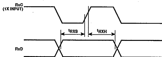
Figure 7. Receive
