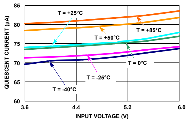
FIGURE 7. QUIESCIENT CURRENT vs INPUT VOLTAGE ( V_{OUT1} = V_{OUT2} = 3.3V , LD01 AND LD02 ENABLED)
