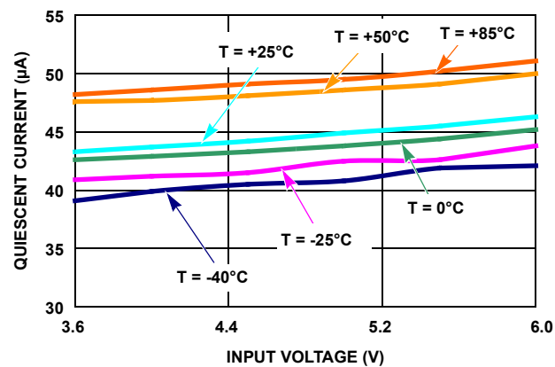
FIGURE 5. QUIESCIENT CURRENT vs INPUT VOLTAGE ( V_{OUT1} = 3.3V , ONLY LD01 ENABLED)
