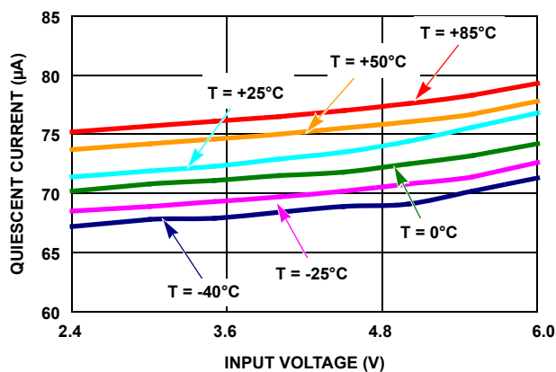
FIGURE 4. QUIESCIENT CURRENT vs INPUT VOLTAGE ( V_{OUT1} = V_{OUT2} = 2.1V , LD01 AND LD02 ENABLED)
