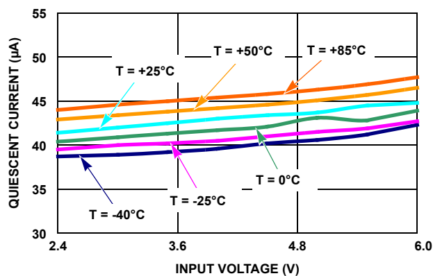
FIGURE 2. QUIESCIENT CURRENT vs INPUT VOLTAGE ( V_{OUT1} = 2.1V , ONLY LD01 ENABLED)
