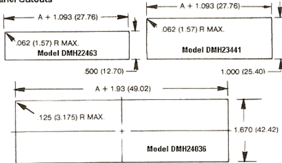
MODELS 22463, 23441
