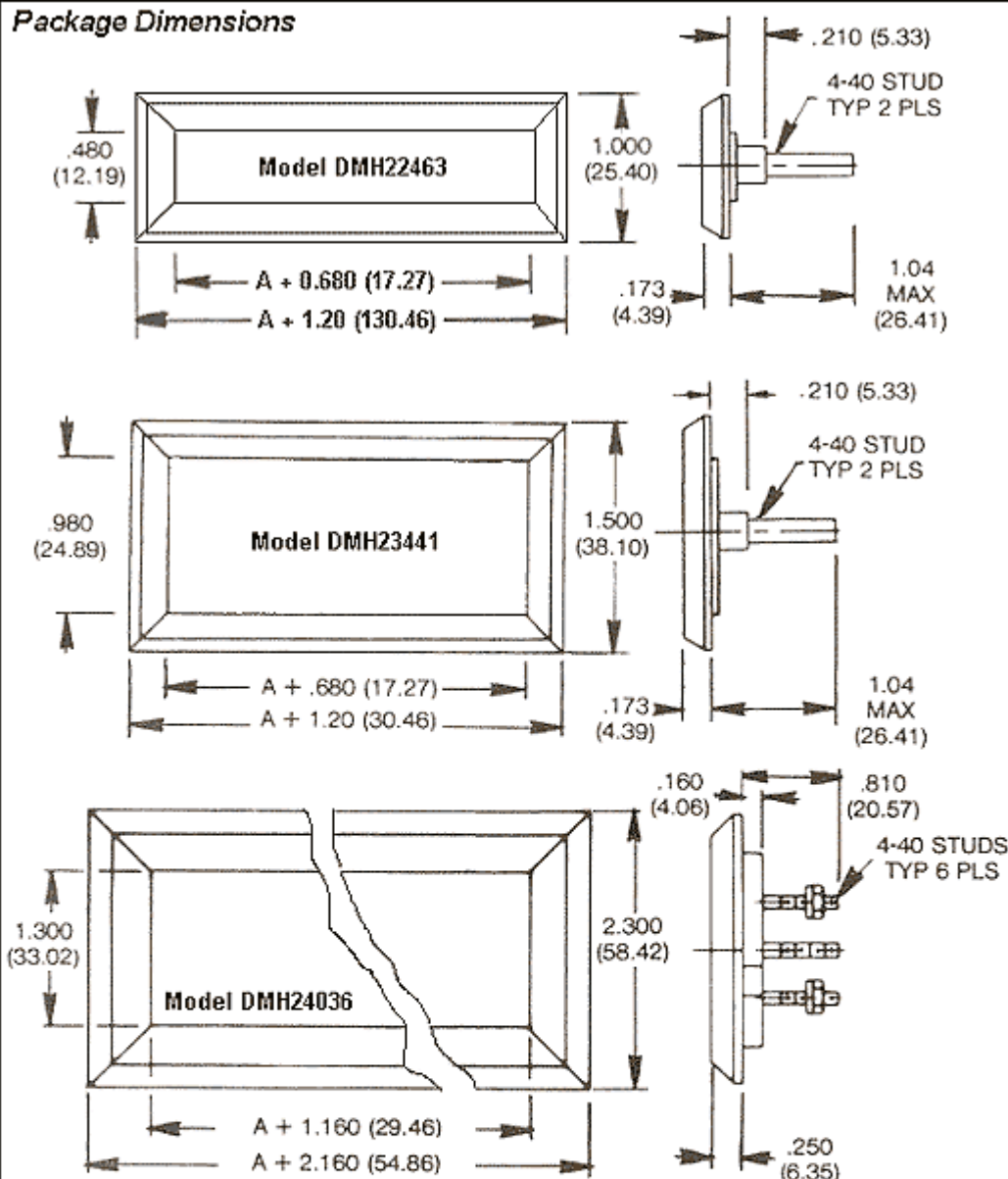
MODELS 22463, 23441
