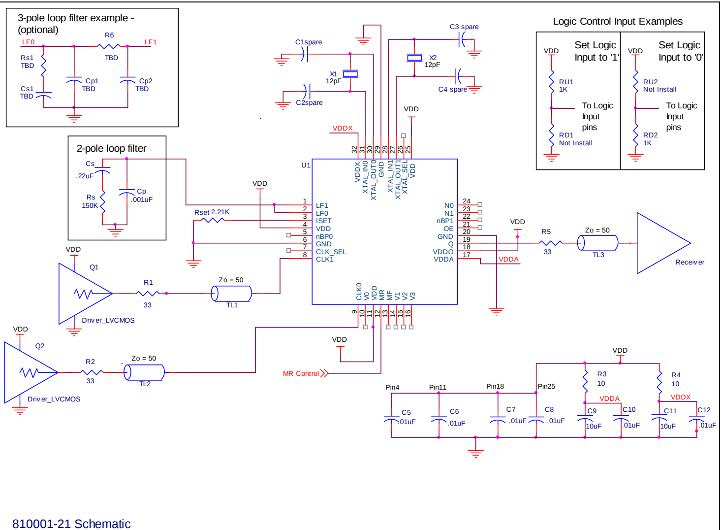
Figure 3. 810001-21 Schematic Example
