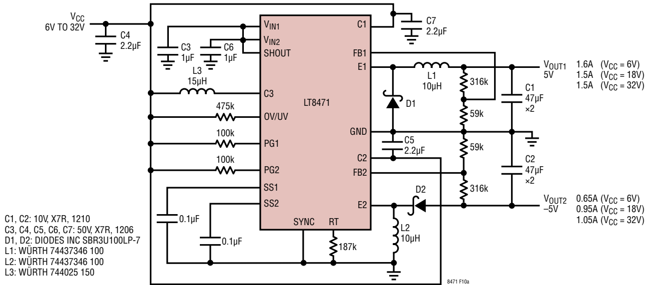
Figure 10a. Wide Input Range Converter with \pm 5V Output Voltages at 450kHz
