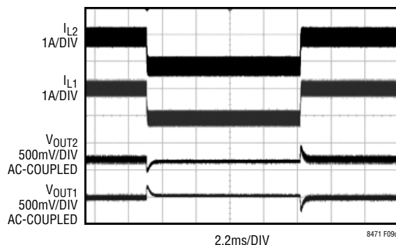
Figure 9d. Load Step Between V OUT1 and V OUT2 from 150mA to 780mA to 150mA (V CC = 18V)
