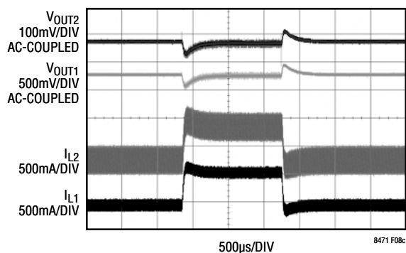
Figure 8c. Load Step on V_{OUT1} from 40mA to 135mA to 40mA
