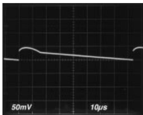
Figure 13. Tantalum Electrolytic
