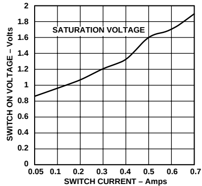
Figure 3. Switch ON Voltage vs. Switch Current in Step-Down Mode
