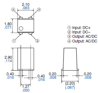
External dimensions
