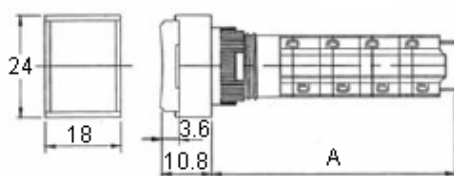
Mounting Dimensions
