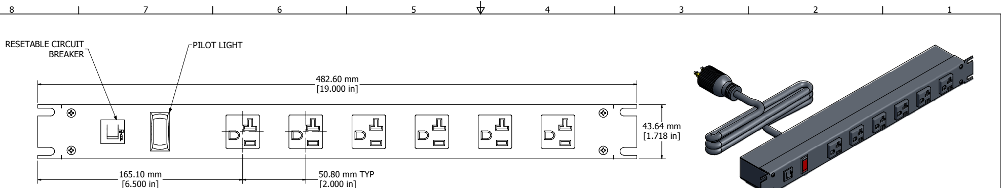
ASSEMBLY - VIEW FROM FRONT
